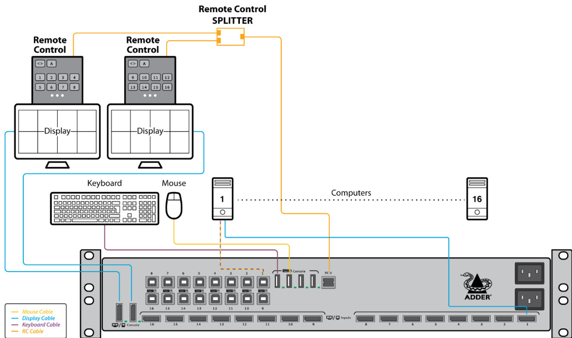
Figure 7 – RCU Splitter Implementation
